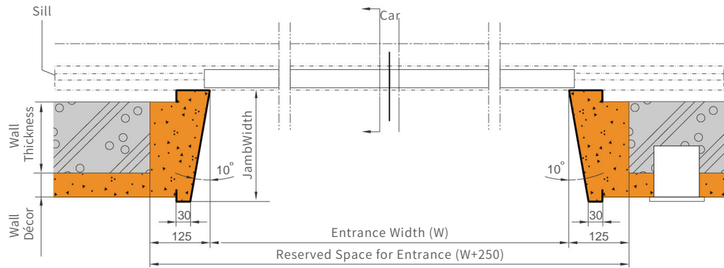
B-B Section
