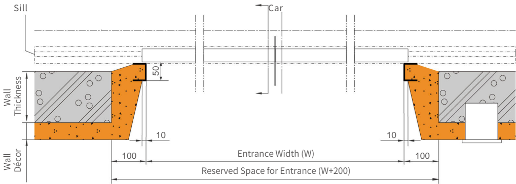
B-B Section
